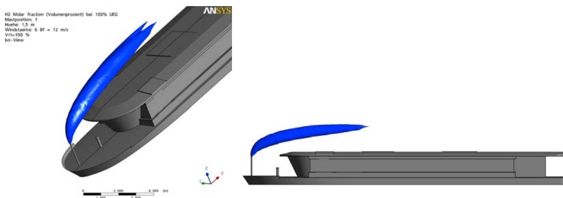
Figure 7. Example of a vent line of an inland navigational vessel
