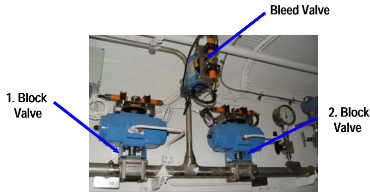
Figure 6. Double-Block-Bleed
