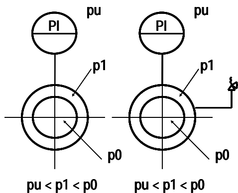
Figure 4. Sketches of Double-Walled-Pipes
